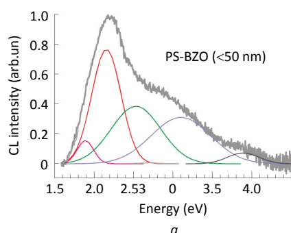
a – composite luminescence spectrum of magnetite-polystyrene \text{BaZrO}_3 ; b – SEM-image of modified magnetite dispersion; c - particles of modified magnetite are attracted by oncological cells, which can be detected by luminescence directly above a magnet
