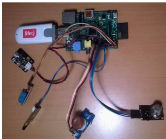
The model of WSN node for the remote sensor-assisted temperature and humidity monitoring
