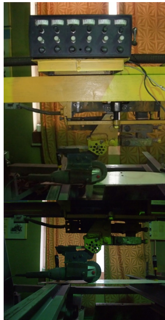
The working equipment fixed on the stand for the surfaces cleaning force measurement
