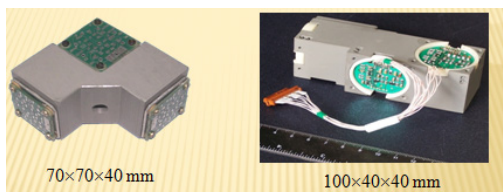
Three-axis variants
