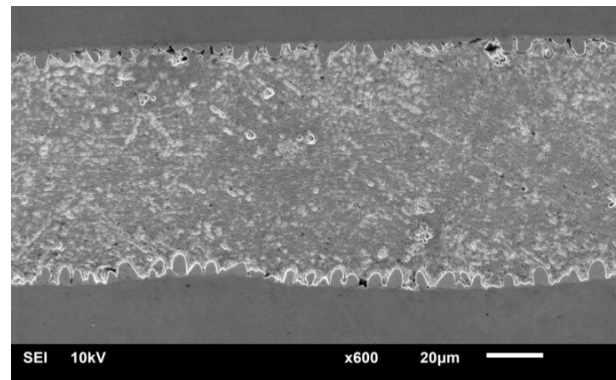
Microstructure of soldered joints in SAC305 alloy with \text{Al}_2\text{O}_3 nanoparticles
