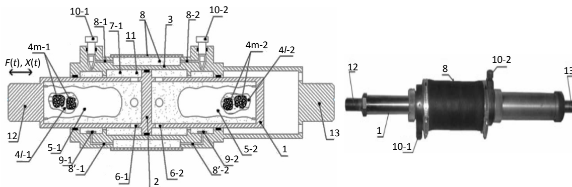
1-rod; 2- piston; 3- cylinder; 4/1, 4/2- working fluid; 4m-1, 4m-2 - porous matrix, 5-1,5-2 – capsules of a heterogeneous working medium, 6-1 ,6-2 ,8-1, 8-2, 8-1`, 8-2`-hydro-channels; 7-1 – working space; 8- balance chamber; 9-1, 9-2 – valves; 10-1, 10-2 – throttles; 11- process fluid; 12, 13 - mounts
