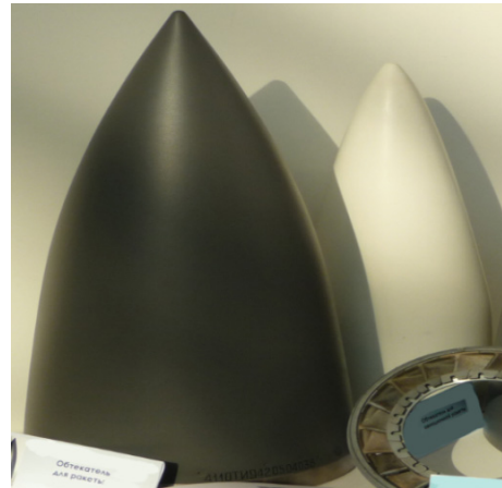
A sample of machined workpiece – the main radio-transparent missile radome
