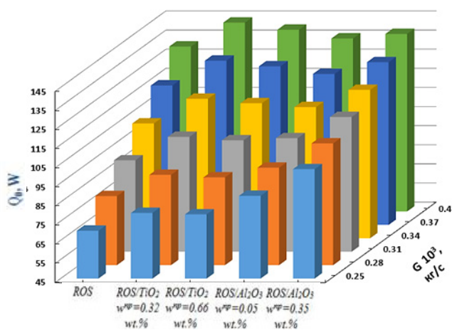
The value of cooling capacity for working bodies (ROS/nanoparticles) at different costs
