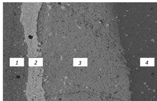
The cross-section of Ti-NbN- overlay on the surface of the cutting element: 1—base; 2 – Ti; 3 – NbN; 4 – \text{Al}_2\text{O}_3
