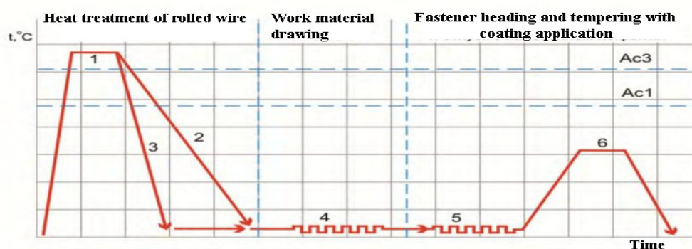
The manufacturing process scheme of high-strength fasteners
