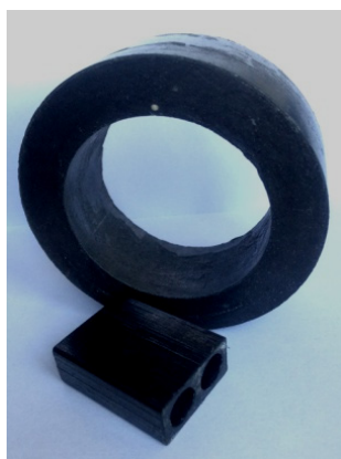
Component parts of the micro-injector MK 10-1 (rotor 90 × 60 × 34, plate)
