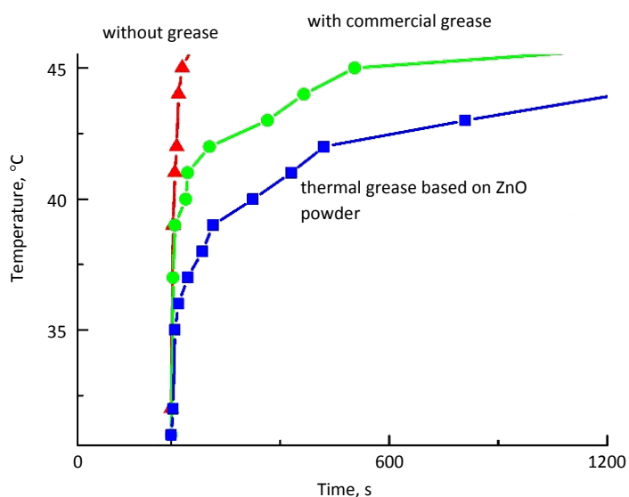
The application of thermal grease in computer technology and graphs of the dependence of operation temperature of the computer processing unit at a steady loading, with copper radiator for heat removal, on the computer operating time
