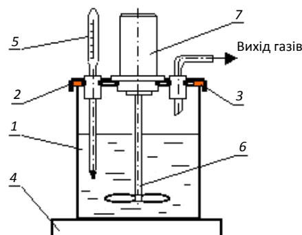
Laboratory equipment for adsorbent production 1 – cup; 2 – lid; 3 – seal; 4 – heater; 5 – thermometer; 6 – stirrer; 7 – stirrer motor
