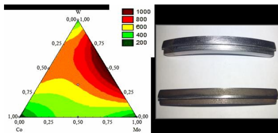
Microhardness (MN / m 2 ) of Co-Mo-W coating for surface reconditioning
