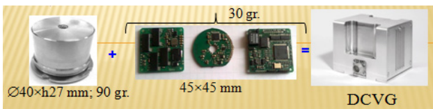
Single-axis unit
